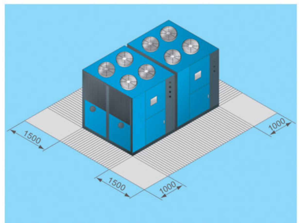
Figure 5a Installation Space Unit: mm
